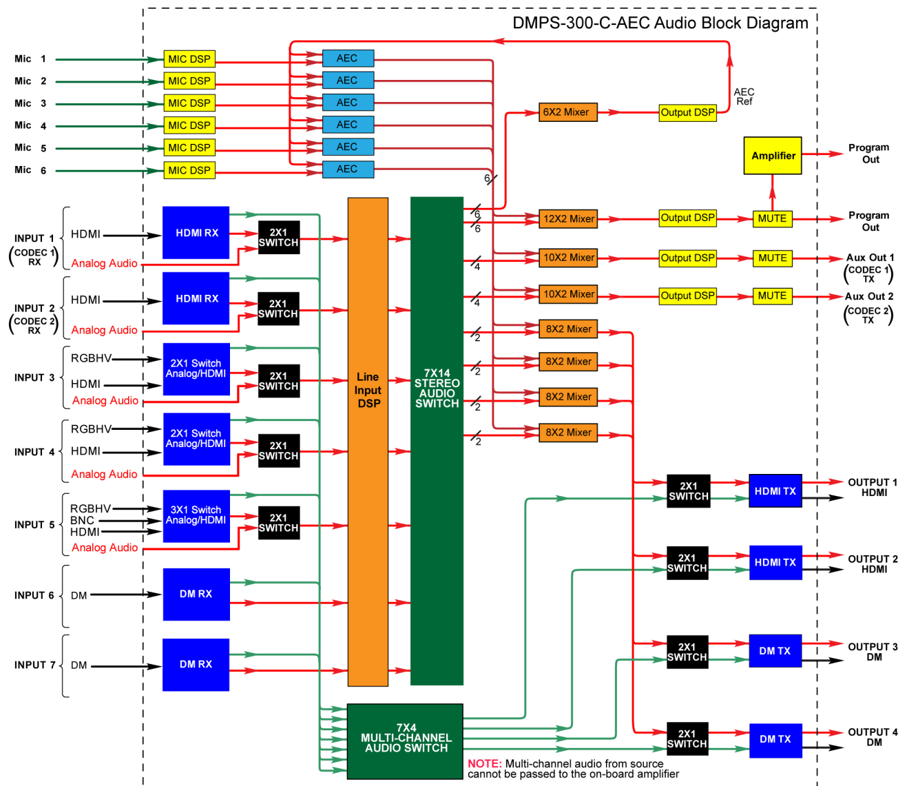
DMPS-300-C-AEC Audio Block Diagram
