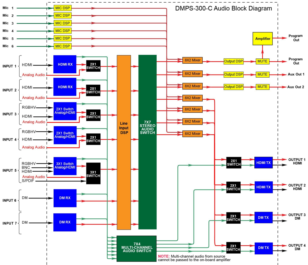
DMPS-300-C Audio Block Diagram
