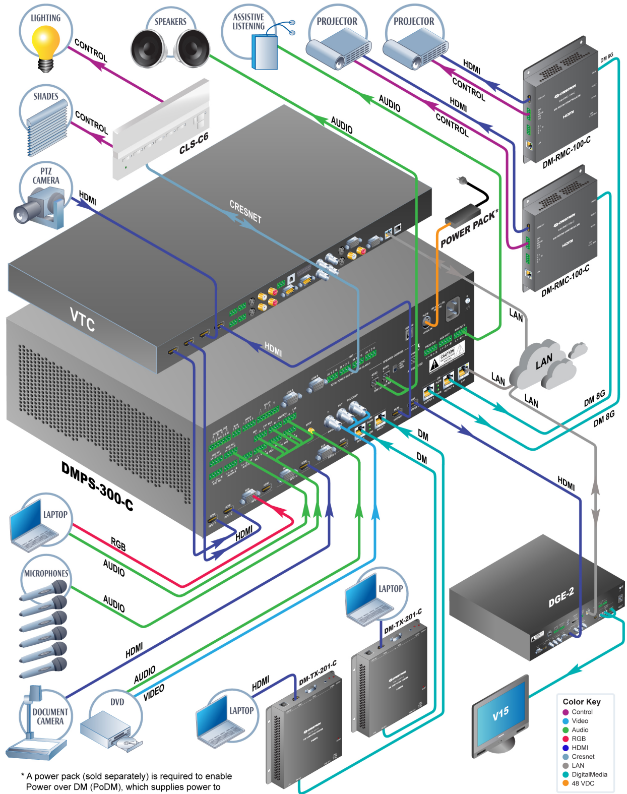
DMPS-300-C in a Video Conferencing Application
