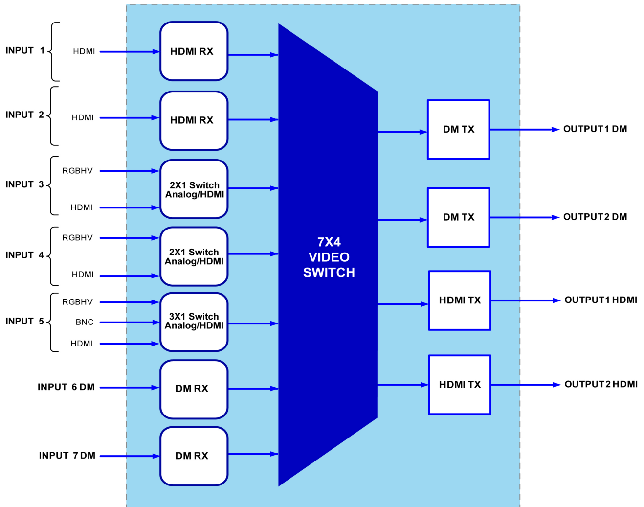
DMPS-300-C Video Block Diagram
